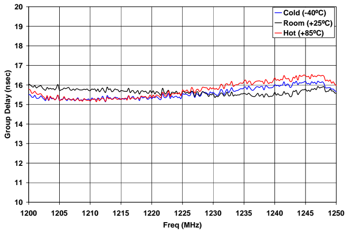
Group Delay @ Maximum Gain
