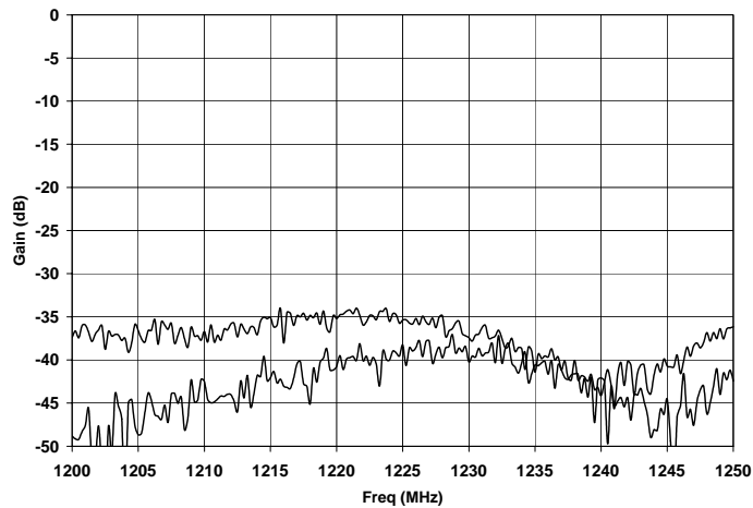
Input to Input Isolation @ 25°C
